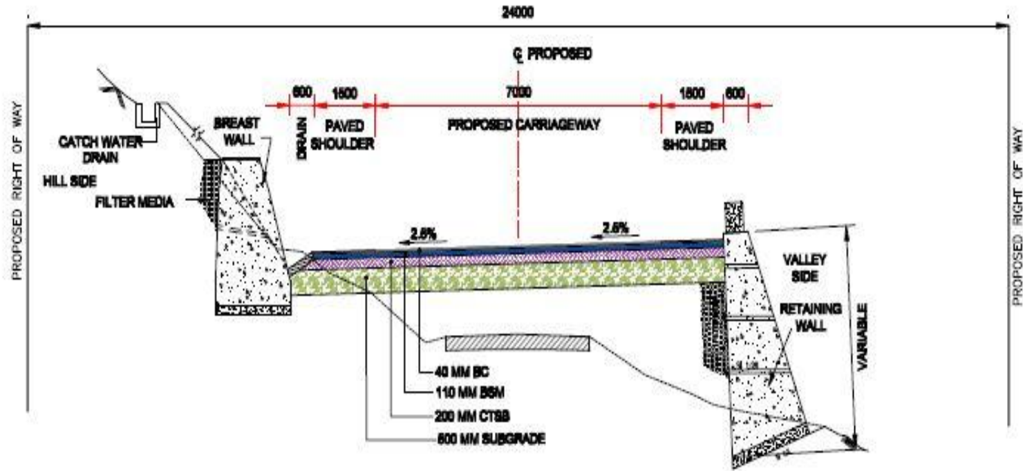
TCS 1 Two Lane With Paved Shoulder Raised Portion(Hill Section)
